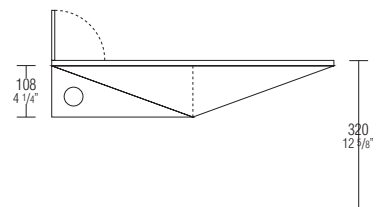
Lateral section
