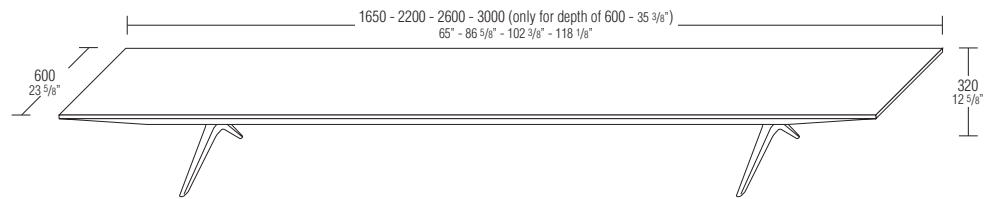
Hi-Tech Bench - D 600 (23 5/8") without wire passage compartment
